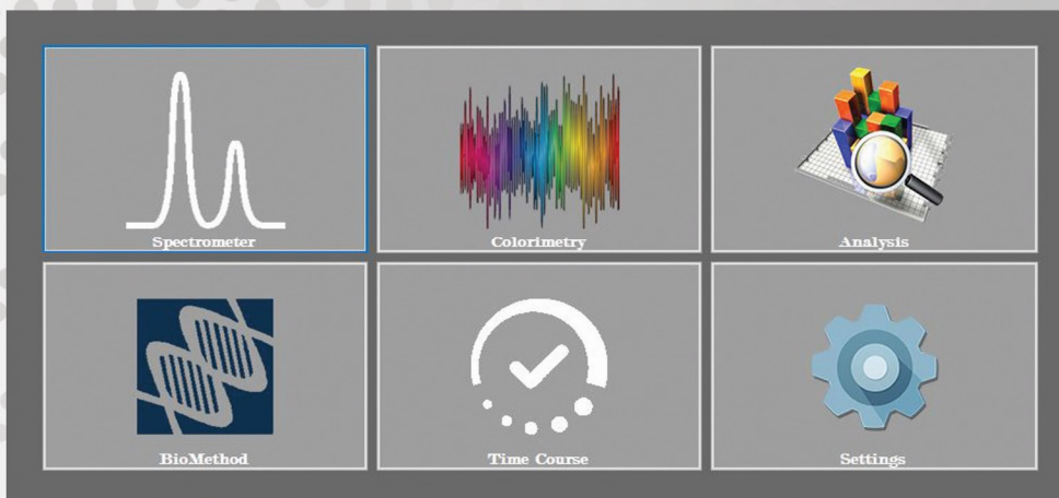
Software Screen
