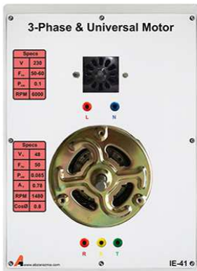
IE - 41 Phase & Universal Motor - 3
