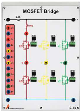
IE - 50 Mosfet Bridge
