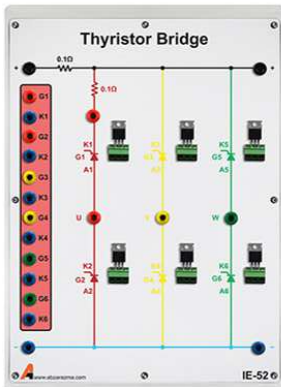
IE - 52 Thyristor Bridge
