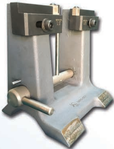
Charpy Fixture
