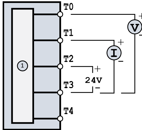
Figure 1 Wiring diagram and terminal assignments
