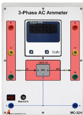
MC - 32 Phase AC Amperemeter- 3
