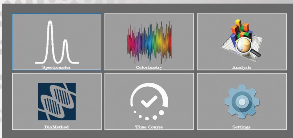
Software Screen
