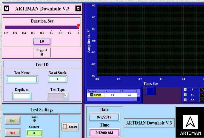
Software Snapshot
