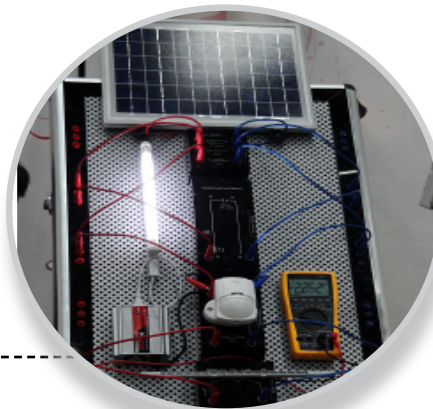
Portable solar training set for AC & DC supply
