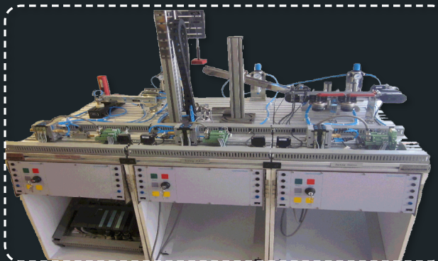
Mechatronics set with 3 stations
